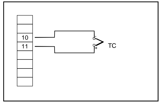
Thermoelement
